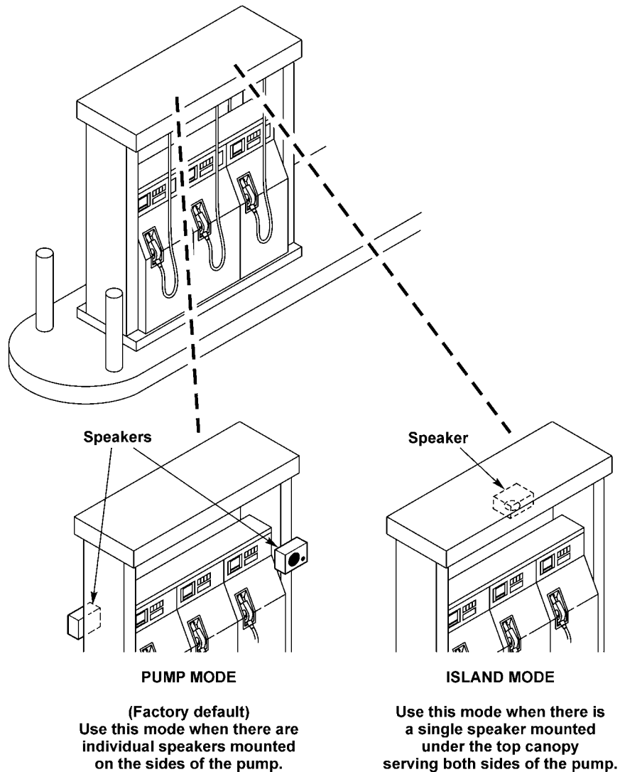
Figure 10. Pump Mode and Island Mode
