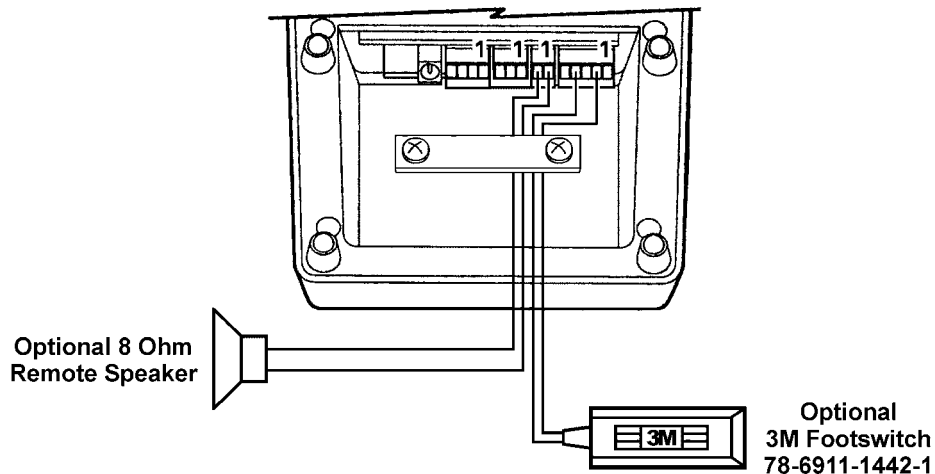
Figure 8. Connecting Optional Accessories to Station Selector
